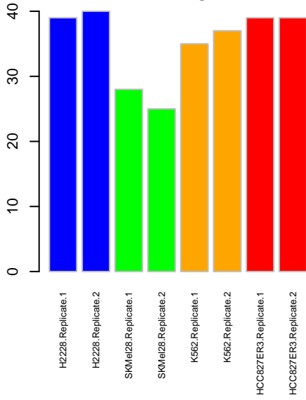
NWK FGR
