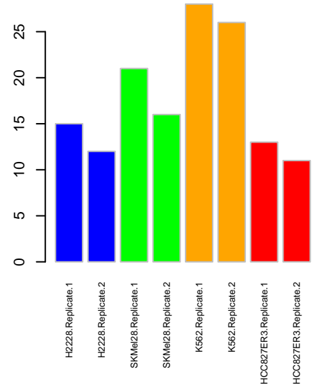
PSP MAPK3
