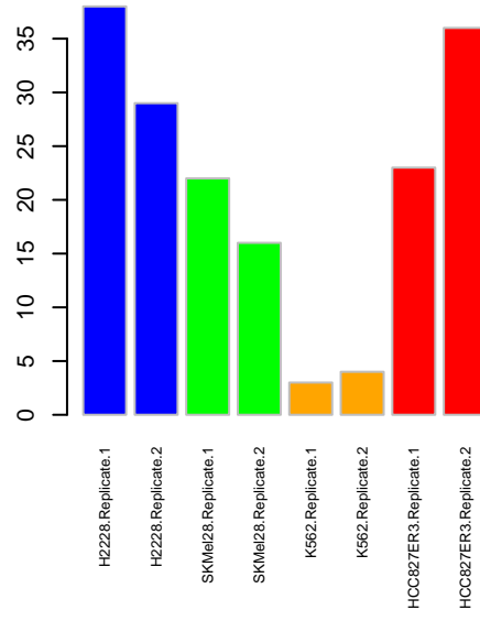
PSP FGR
