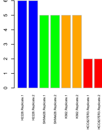
PSP PRKACA
