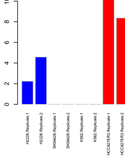
InKA EPHB3
