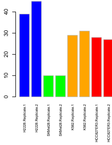
PSP ALK
