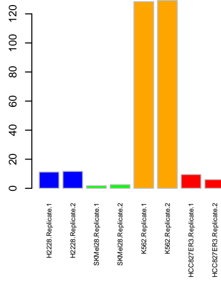
InKA ABL2
