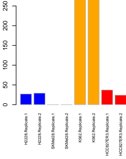
InKA ABL1
