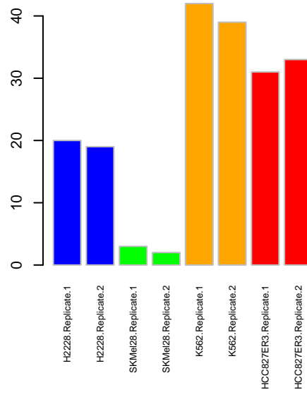
NWK FLT1
