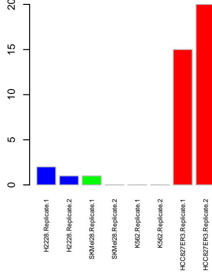
NWK STK11
