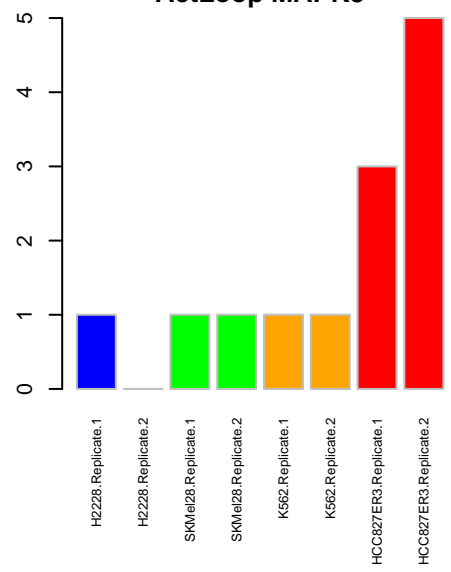
ActLoop MAPK8
