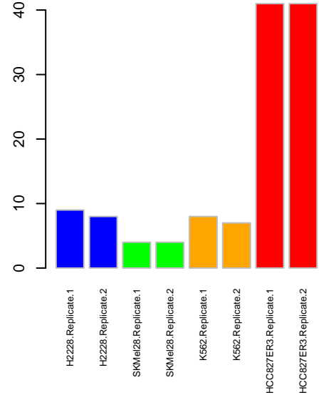
NWK ERBB3
