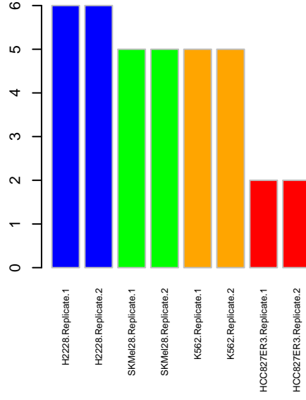
ActLoop LCK
