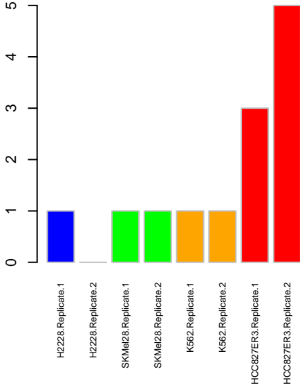
NWK MAPK10
