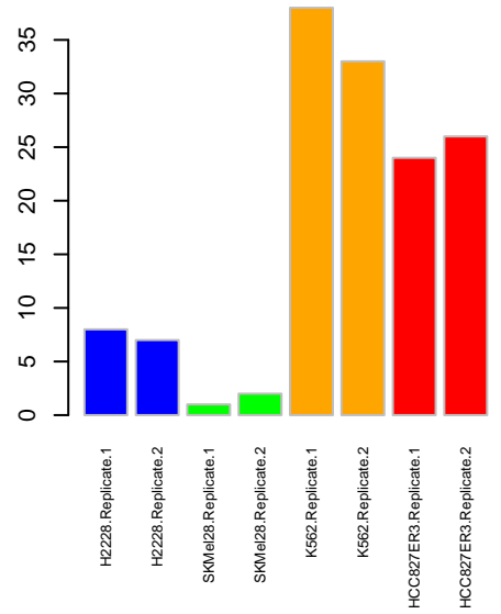
NWK MAPK1
