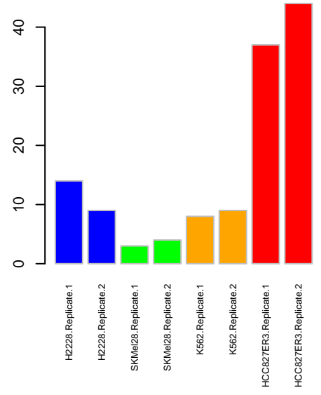
NWK LCK
