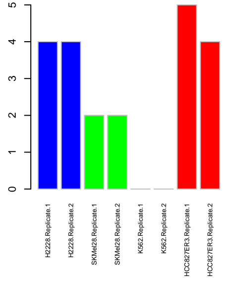
PSP YES1
