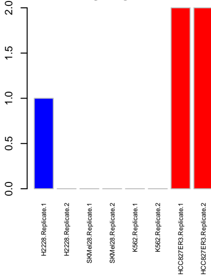
PSP TGFBR2
