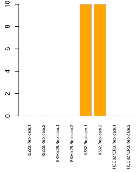
PSP TEC
