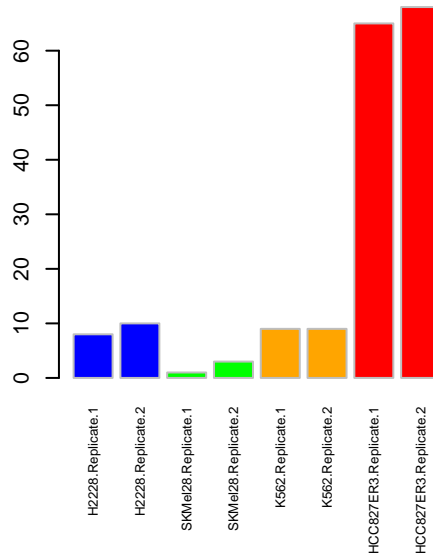
NWK ERBB4
