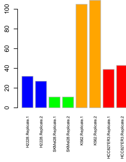
NWK KIT
