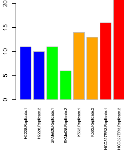
Kinome TNK2
