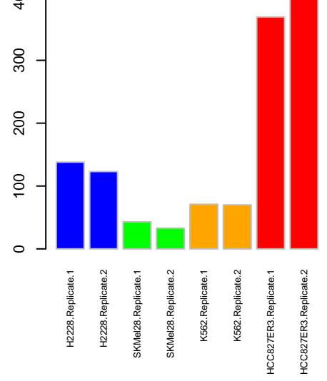
NWK ERBB2
