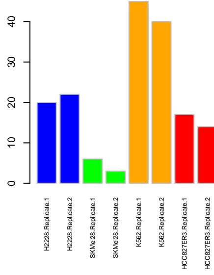
NWK TEC
