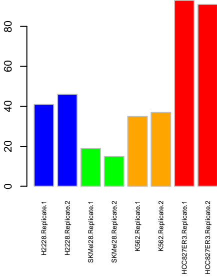
NWK YES1
