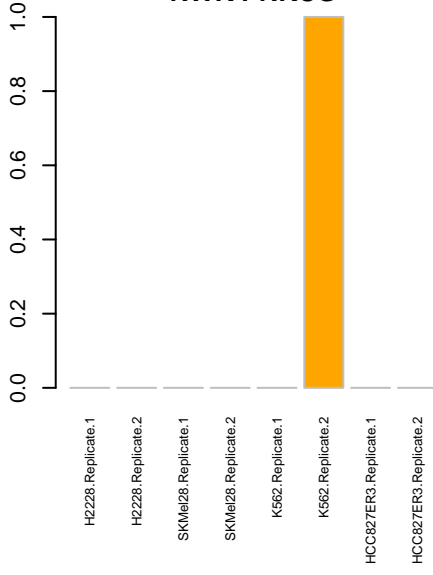
NWK PRKCG
