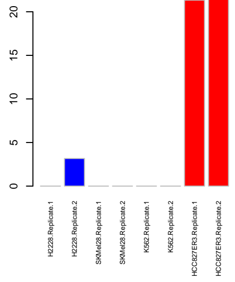
InKA ERBB4
