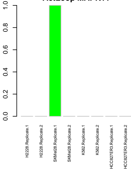
ActLoop MAPK11
