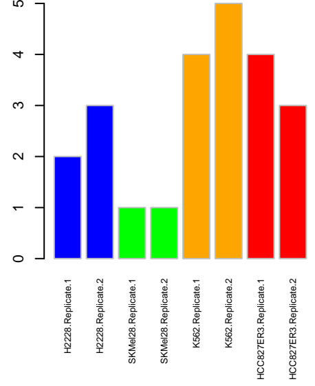
NWK PTK6
