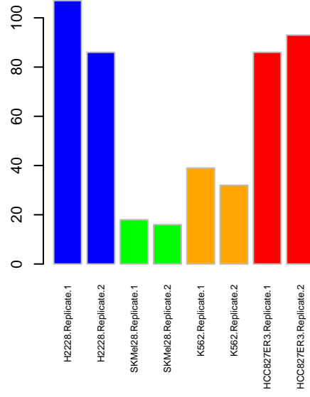
NWK INSR
